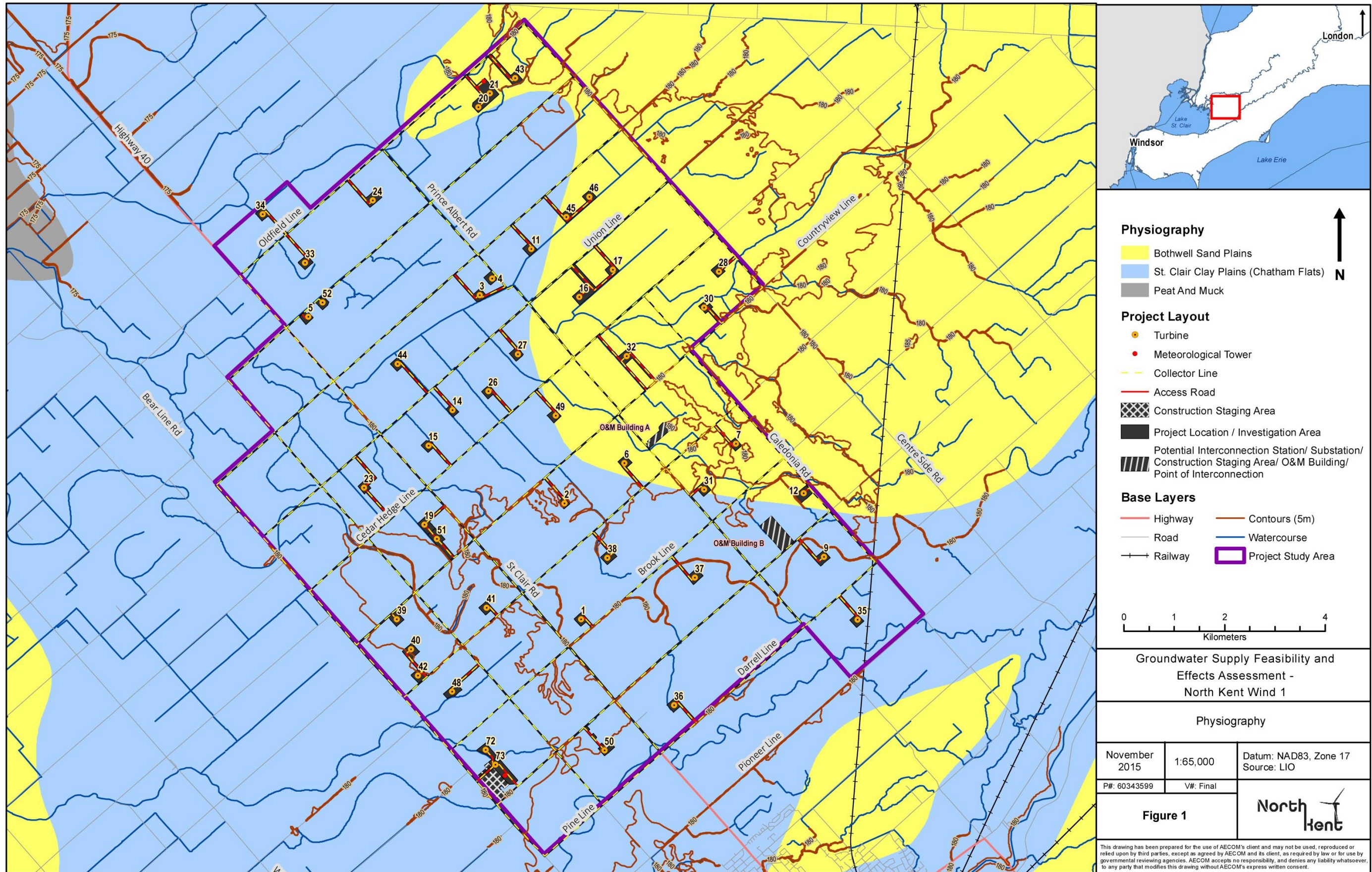
Figure 1: Physiography
